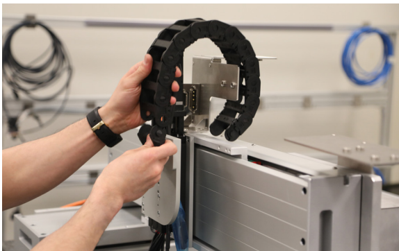
Fig. 4 Attaching the cable chain
